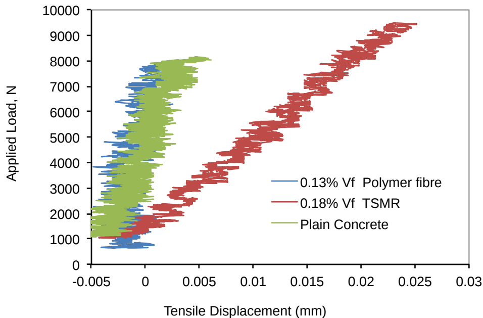
Figure 3. TSMR 5-25 Tensile Stress Strain (5)
